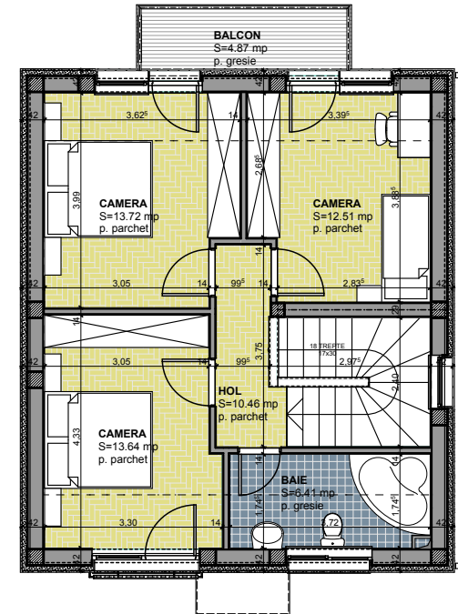
PLAN MANSARDA
