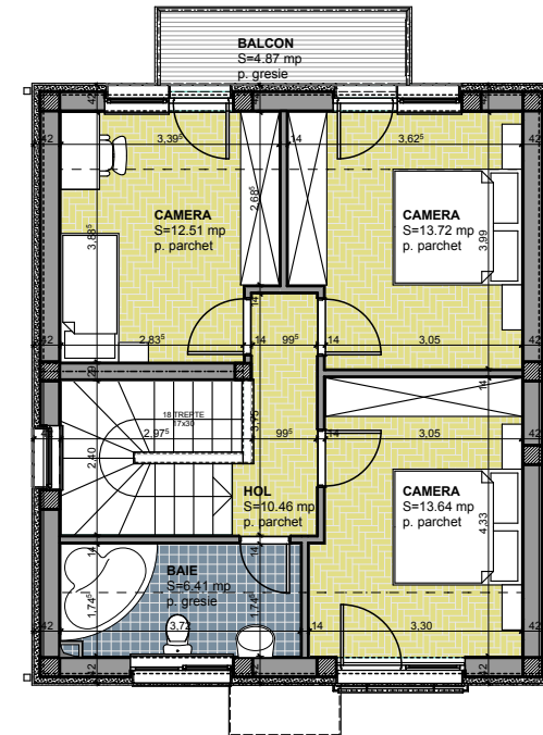
PLAN MANSARDA
