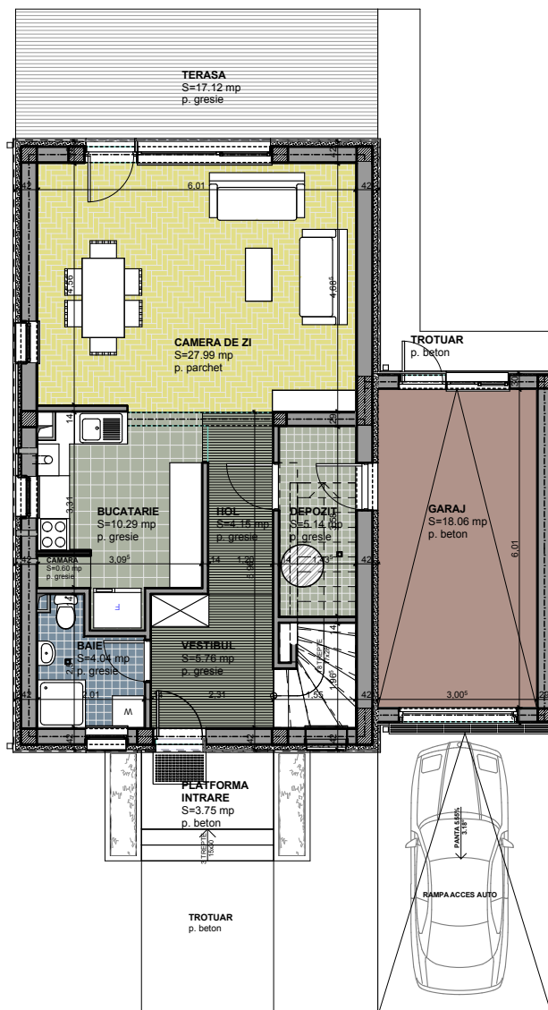
PLAN PARTER
