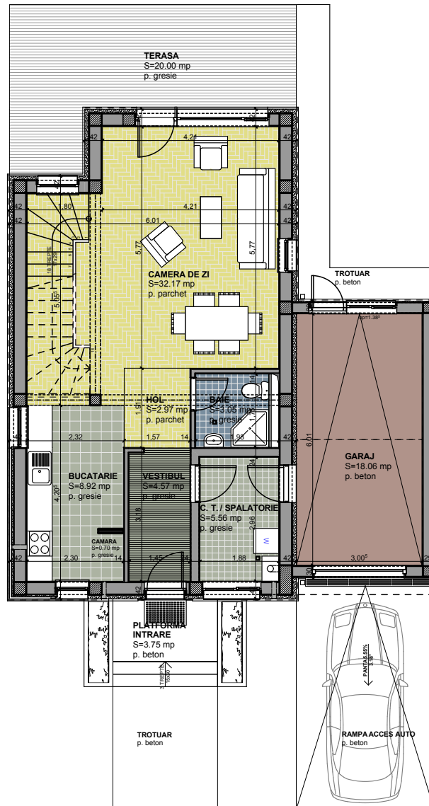
PLAN PARTER
