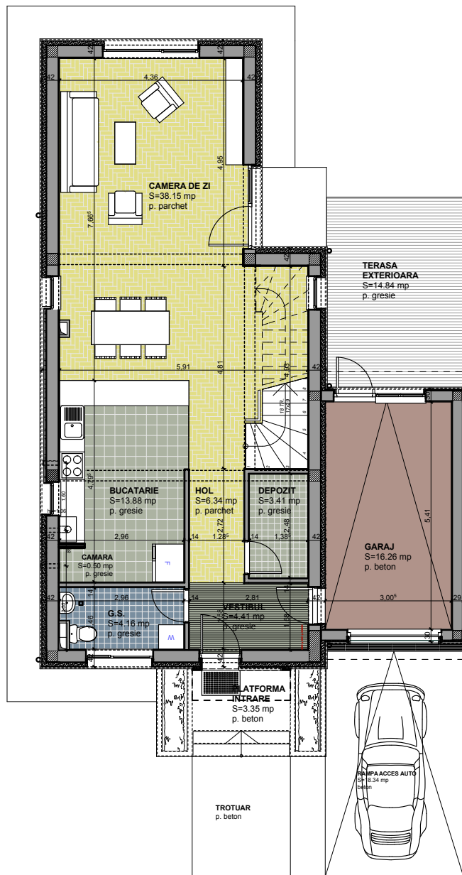
PLAN PARTER
